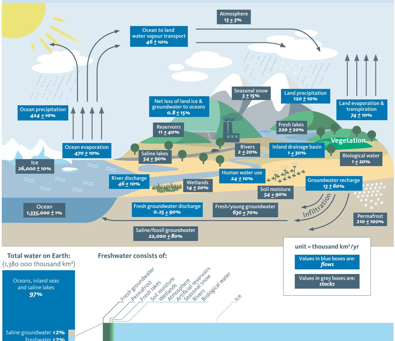
Figure 2.1. The global water cycle with estimates of water flows and stocks. Source: Kerres et al. (2020).
