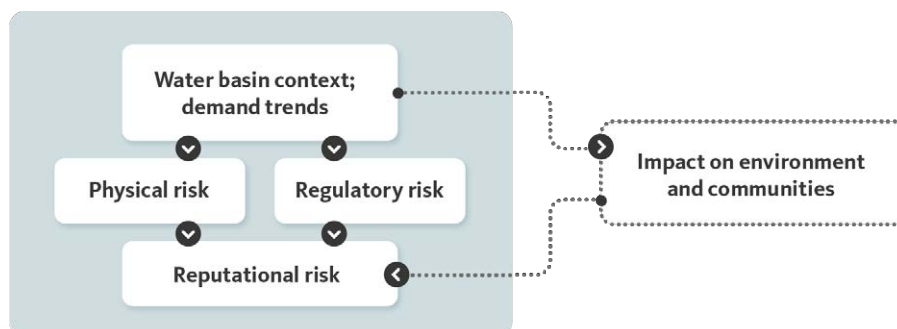
Figure 1: Water Risks
